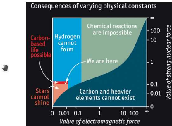
Figure 2. Fine-tuning of the parameters \alpha and \alpha_s . Life-permitting parameter zone of these constants is marked in red [65].
