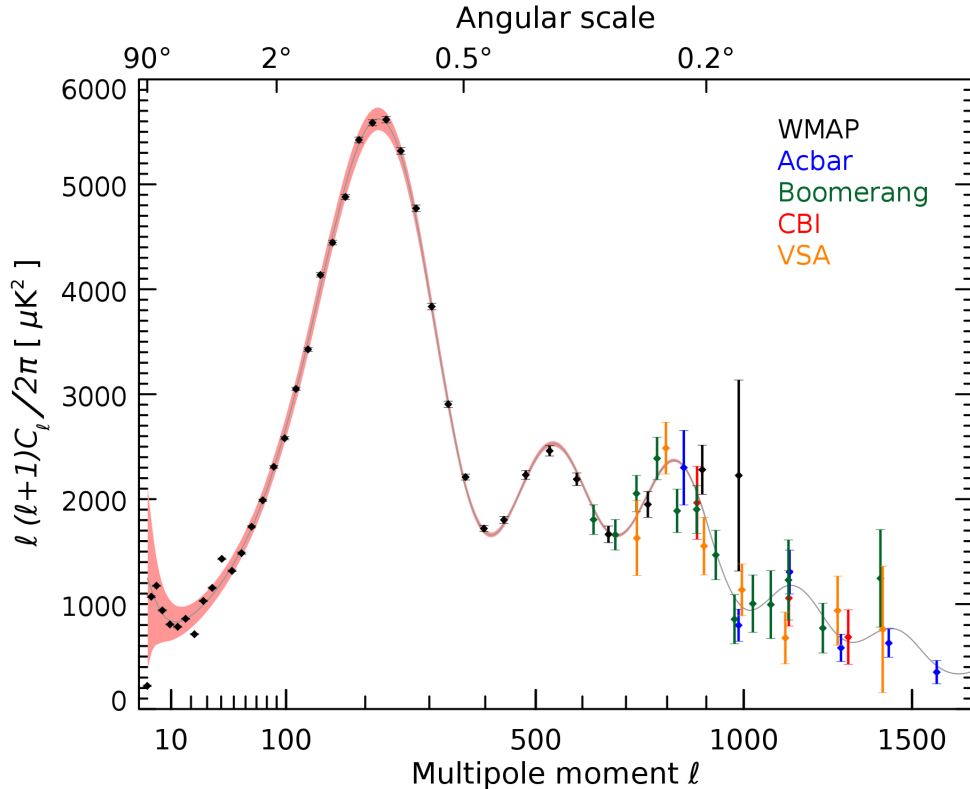
Figure 2: Anisotropies of the CMB power spectrum, by different cosmological observations and satellites.
