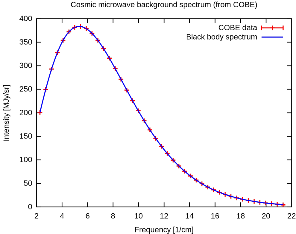
Figure 1: CMB spectrum captured by the COBE satellite. It corresponds to the spectrum of a hot black body with a temperature of about 3 K.
