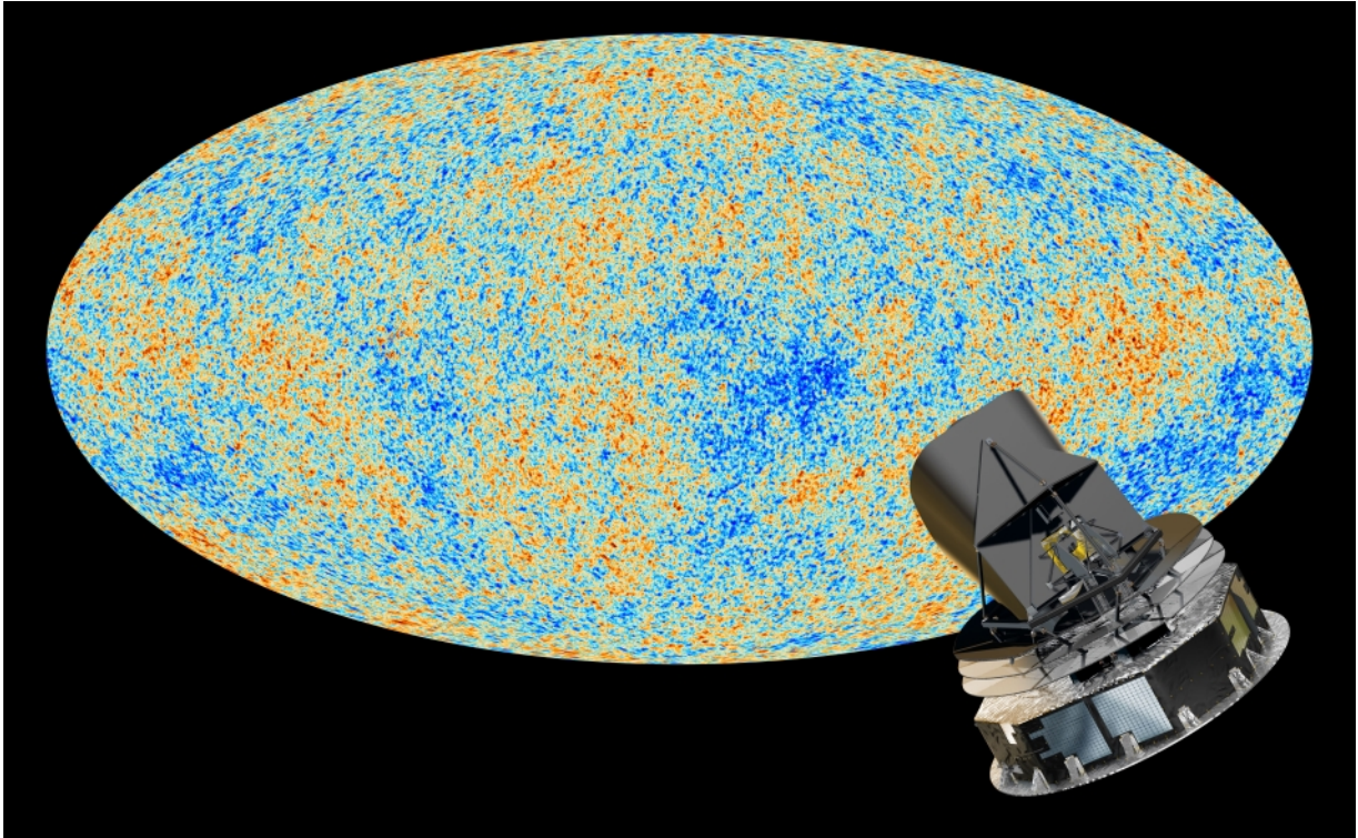
Figure 3: The most accurate CMB map is from the Planck (ESA) mission.
